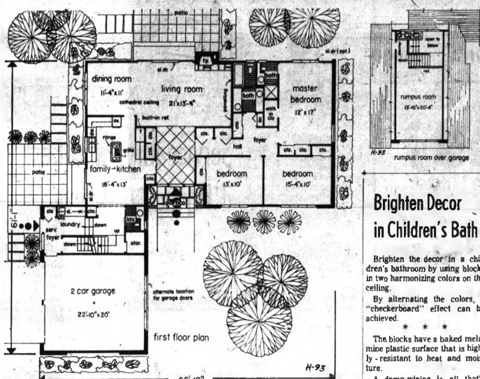
FLOOR PLANS —Excellent separation of three main areas of this ranch is readily apparent. Take special note of the large, formal entertaining area at the rear.
