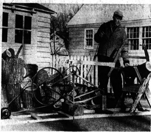
BUCKING UP — Frank L. Anderson, St. Paul, Minn., saws firewood for Christmas with his homemade bucksaw. Small electric motor (lower left) turns rear wheel on inverted bike,
