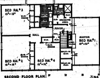
FLOOR PLAN — House contains 3,600 square feet of living area on first floor not counting 67-square-foot screened porch and 505-square-foot garage. Second floor contains 1,208 square feet. Dimensions are 78' wide by 34'8" deep overall.
