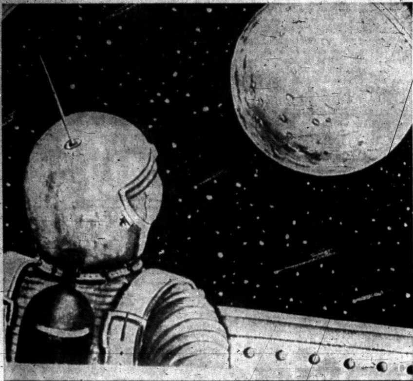
NEARING MARS — AP artist John A. Carl-ton's drawing shown here is a conception of the view from a space ship on its way to Mars. The human passenger, wearing a special pressurized space suit gazes through a porthole into black space crowded with meteors and brilliant stars.
