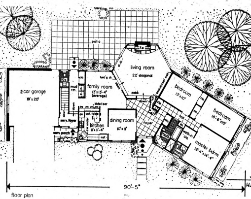
FLOOR PLANS —Note the excellent traffic circulation of this unusual design, with easy movement from the foyer to any part of the house, as well as from the service porch to the patio.
