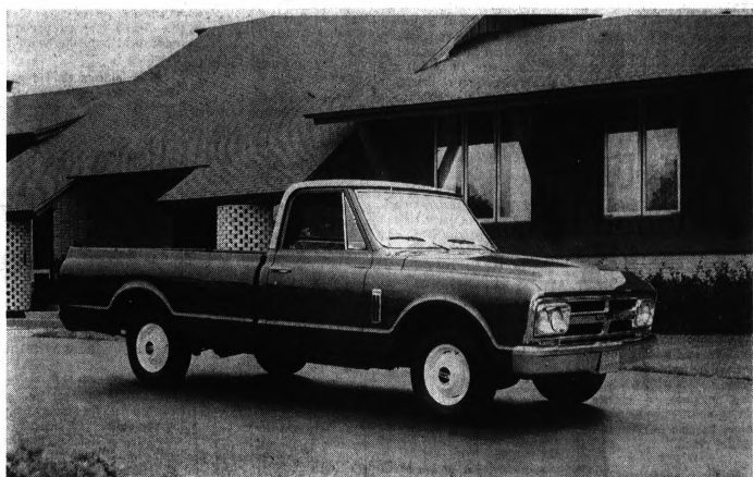
NEW GMC V8s — Light trucks similar to this three-quarter-ton pickup are now being powered by two new V8 engines introduced today by GMC Truck and Coach Division. One of the new V8s is a 283-cubic-inch unit developing 175 horsepower and the other is a 327-cubic-inch version with a 220-maximum horsepower.
