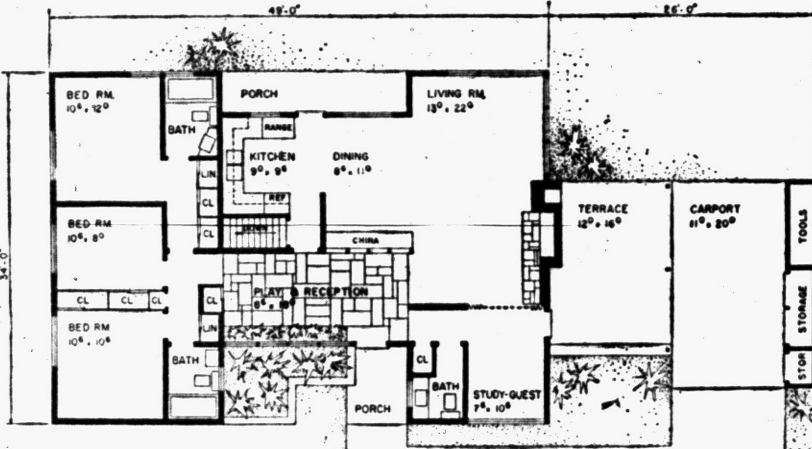
PAVED RECEPTION ROOM, fronted with floor-to-ceiling windows, is a feature of this plan. Broken line shows folding partition between living room and study.
