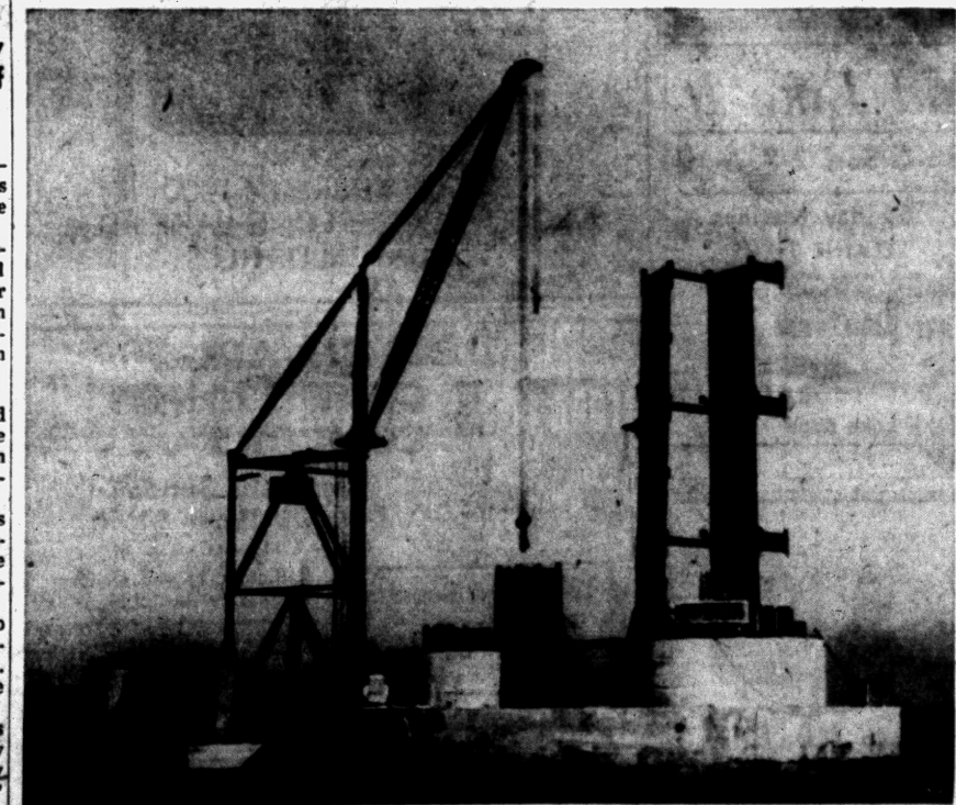
TOWERS TAKE FORM — Towers for the main span of the Straits of Mackinac bridge begin to jut into the sky as the second phase of the construction of the big bridge is started. A gantry crane is lowering a second base plate at pier 20 on the north side of the straits as bridge steel workers take over from the general contractors for the construction of 33 piers that will carry the bridge across five miles of water.
