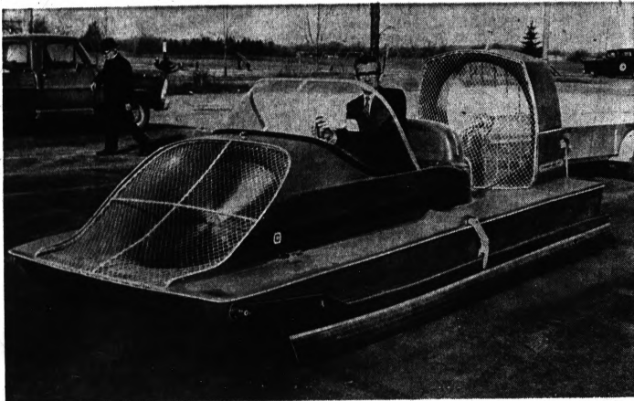
RIDES ON AIR —Dan Berry of Sports Hover Craft, 2520 Airport, Waterford Township, demonstrates the Cushionflight 240, a novel craft that rides on a cushion of air over land or water. The craft, which holds two adults, is made of fiber glass and reaches speeds of 35 miles per hour.
