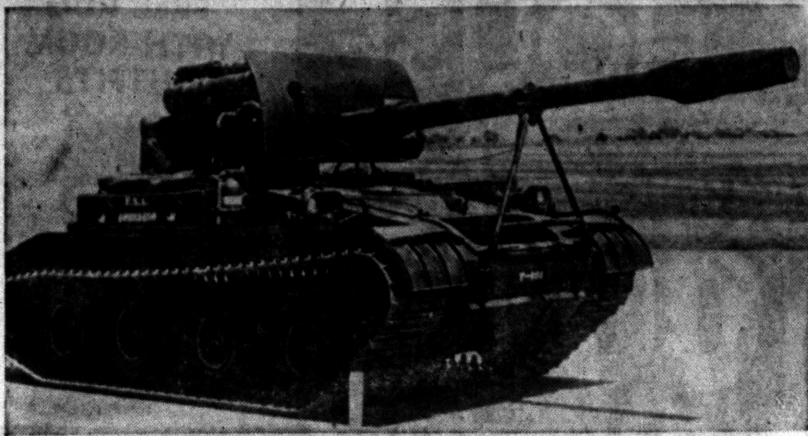
PUNCH WITH ITS OWN POWER — It looks like a tank, but it isn't. It's the just-unveiled T-101, a 90-mm. self-propelled gun. A powerful antitank weapon, it is light weight, enabling it to cross muddy, marshy or sandy terrain. It can also be air-dropped. Designed for use in the assault phase of airborne operations, the T-101 carries a three-man crew. Its armament is mounted above the hull without a turret. Department of Defense photo taken in Washington, D. C.
