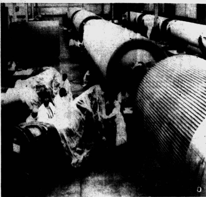
TAKE THE WRAPS OFF MISSILES—Assembly line employees at the Chrysler missile plant at 16-Mile and Van Dyke, Sterling Township, move Jupiter engines (left foreground) into position for installation into the missile's booster section during final assembly operations. In right background is a Redstone final assembly line. The plant, previously top-secret, was opened for a newsmen's tour today.
