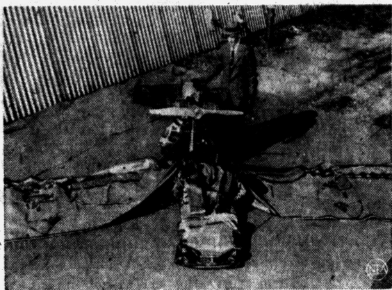
flatplane is ready to be inflated. Wing and tail assembly are made of rubberized Airmat, fuselage is airship cloth.
