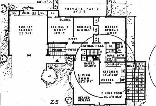
FLOOR PLANS: L-shape permits three bedrooms and garage along rear portion of house, with living room, dining room and kitchen at the front—all tied together by a foyer
