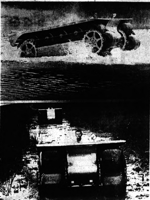
THE AIROLO—Shown undergoing tests, this tractor-type vehicle with 26 balloon-like wheels will soon be carrying U.S. Marines and war supplies through anything—even quicksand. A product of the Ingalls Kalamazoo Division
