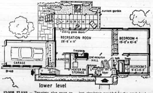
FLOOR PLANS — Two-story plan saves on building costs, but complete ranch-style living facilities are provided on upper level. Note excellent circulation provided by the grade-level entrances.
