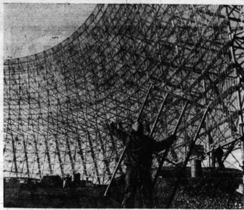
SETTING UP SCREEN — Workman carries steel frame, one of 2,000 used to build giant detection radar antenna at USAF base in Thule, Greenland. Antenna is one of four at Thule capable of detecting missiles 3,500 miles across the Arctic.
