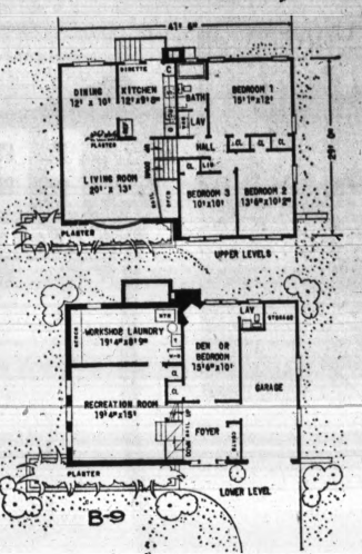
FLOOR PLAN — Plans show arrangement when entrance is on the ground level, making possible big foyer to channel traffic. Balcony rail in living room overlooks the foyer.
