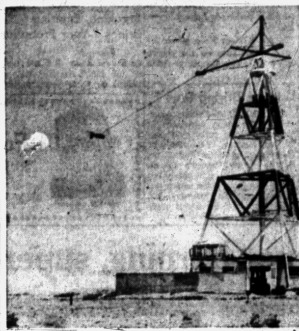
"CHUTE" THE WORKS —In order to find out what happens when a pilot bails out at 500 mph, the Air Force constructed this instrument at El Centro, Calif. Called the Whirl-Tower, it releases parachutes with instrumented dummies at subsonic speeds, attained through centrifugal force. At a predetermined speed the parachute and dummy are released from the rotating boom. Sensitive instruments and photographic equipment record effect of fall.
