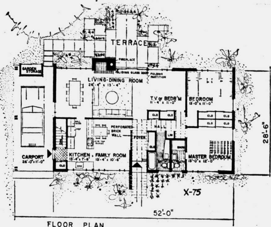
FLOOR PLAN
