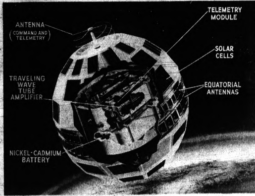
TELESTAR — This cutaway drawing shows the devices contained in the communications satellite sent into orbit early this morning. This country's first privately owned space vehicle will test the feasibility of relaying intercontinental telephone and video signals via a satellite network.
