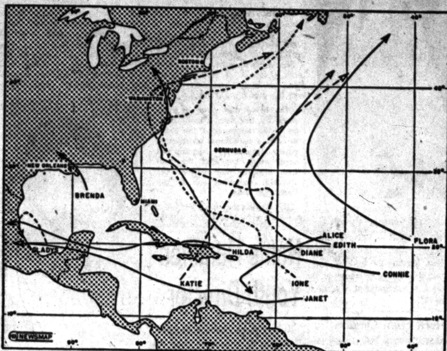
1955's STORMY WEATHER—The chart above shows the paths of last year's hurricanes. The 1956 season began June 15 and will last through the middle of November. U. S. weather experts are currently plotting the course of all this year's "girls."
