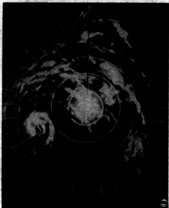
EYE OF A HURRICANE—Here's what the big wind looks like on a radar scope. What you're looking at is the swirl of rainfall into the eye of hurricane Connie off Cape Hatteras, N. C., last August. The eye is at lower left, about 65 miles from Hatteras (in the center of the scope).
