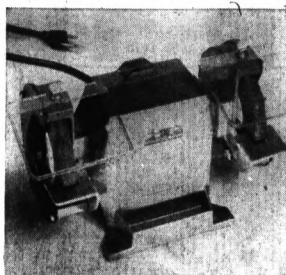
AMC 4\frac{1}{2} " bench grinder has a 3450 f.p.m. motor, 2 grinding wheels, eye shields, plus handy tool rest . . . 19.99
