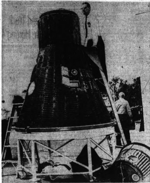
INSPECTING MERCURY CAPSULE — National Aeronautics and Space Administration technicians inspect the Mercury capsule that survived a tortuous 12,500-mile-an-hour rocket ride Tuesday. A periscope protrudes from door at center. The scorched antenna canister removed from the top of the capsule is at right. This inspection is being done at Cape Canaveral, Fla. The Tuesday flight was a test for the Astronauts, possible in April.
