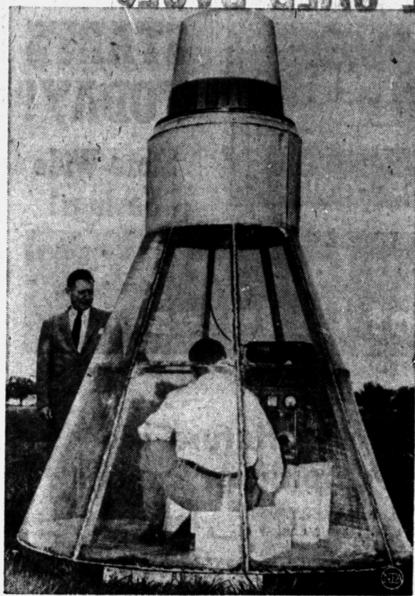
MERCURY MOCKUP — The possible home of a future space-man, this object is a full-scale antenna-test mockup of a Project Mercury capsule. Engineers are shown testing the complete communications system for the capsule in Cedar Rapids, Iowa. Objectives of Project Mercury are to put a man into space, recover the capsule and its occupant and investigate the capabilities of man in this new environment.
