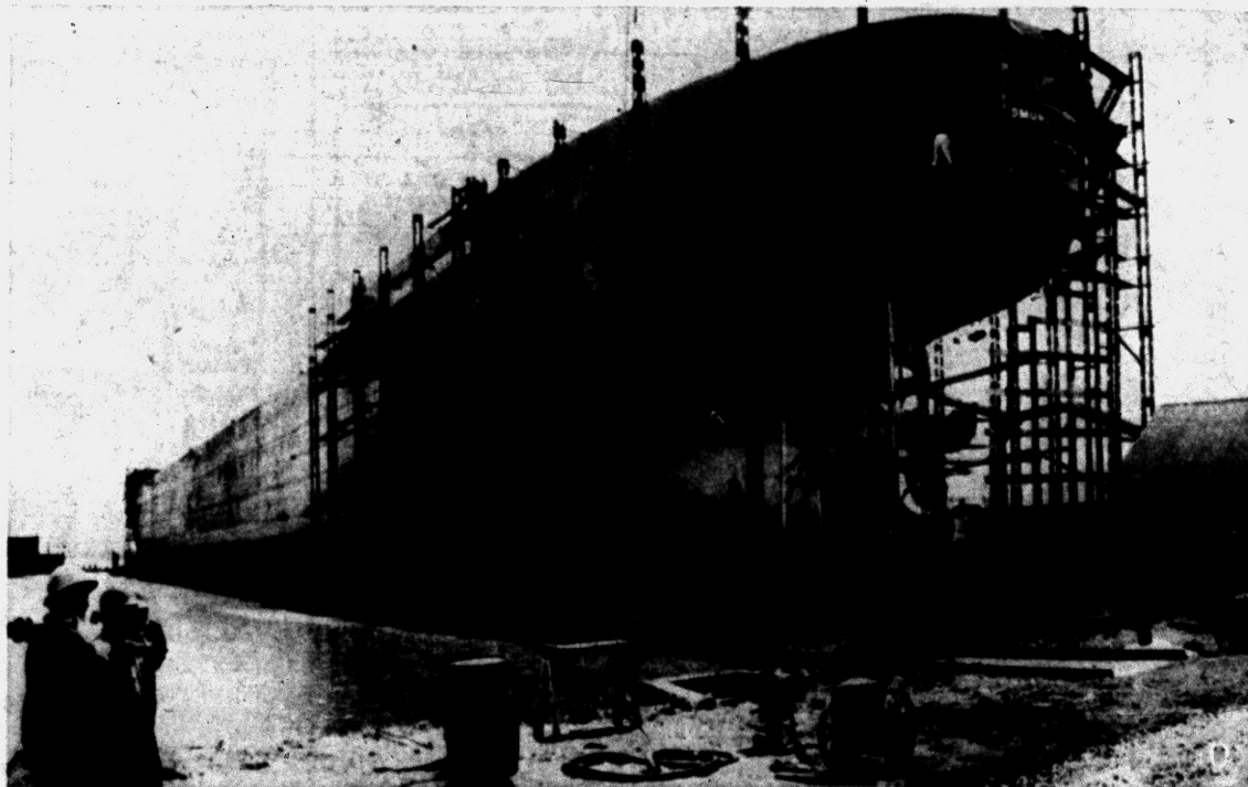
729-FOOT GIANT — The longest and largest ship ever built on the Great Lakes will be launched tomorrow in River Rouge. It is the ore carrier S. S. Edmund Fitzgerald, 729 feet long, 75 feet wide and weighing 7,500 tons. It is longer than Detroit's 47-story Penobscot Building is tall. The eight million dollar ship is 13 feet longer
