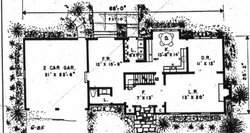
FLOOR PLANS: Excellent circulation pattern of first floor is typified by strategic location of laundry-mud room between family room and kitchen, with a door from the rear
