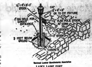
Illustration of a lawn lamp post construction. The post is 8 feet long, with 3 feet under ground, leaving a 5-foot length to the cap. Square the ends of the four pieces, using a miter box. If the post is to be made square in cross-section, as shown in the drawing, rip two of the pieces of 1 1/2 by 4-inch stock to a width of 1 1/4 inches, and plane the edges.
