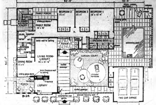
FLOOR PLAN — A host of outstanding details make this home distinctive. It's designed to provide for every kind of family activity, including the most lavish entertaining.
