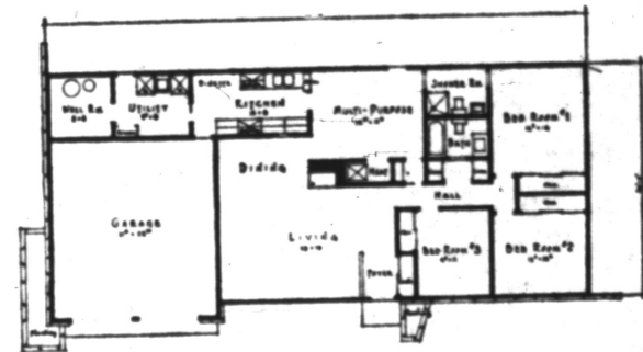
FLOOR PLAN
