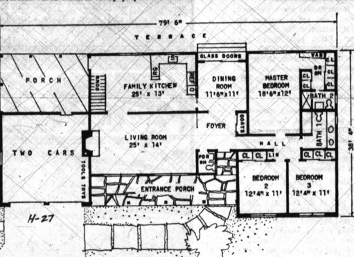
FLOOR PLAN — The basic living area is 1,848 square feet. Good planning keeps hall space to a minimum yet provides easy movement from one part of the house to another. Note also the copious closet space.
