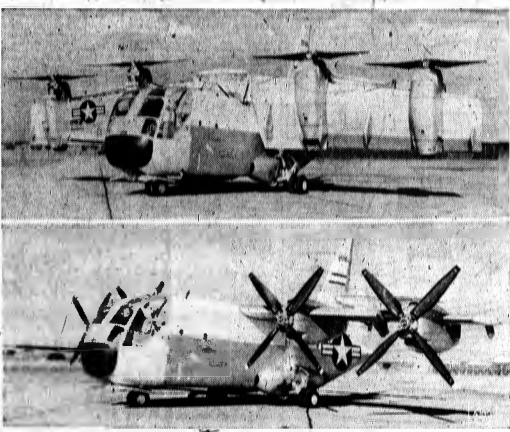
HALF-SMOKED CIGAR — That's one of the names the Air Force's experimental vertical takeoff plane has been given. When they swing level.
