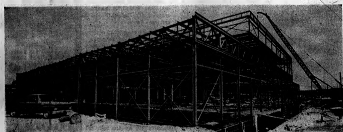
Foundry Addition At Pontiac Motor Division Will Cover 180,000 Square Feet
