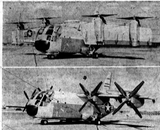
HALF-SMOKED CIGAR—That's one of the names the Air Force's experimental vertical takeoff plane has been given. When heading for the clouds or down to earth, the craft's wings pivot upward. For straight flight they swing level.
