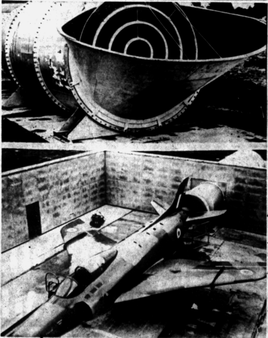
JET SILENCER—The problem of quieting the ear-splitting roar of jet engines was met with a giant muffler at the South Marston plants of Vickers-Armstrong, England. The plane to be tested is moved into the walled-in pen with its tail section in the exhaust muffler. A close-up view of the muffler is shown at the top. It is so efficient that it reduces the noise level to a point where it is practically inaudible at 1,000 yards.
