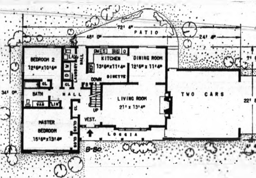
FLOOR PLANS: Center hall planning in both the front and rear is the key to excellent circulation in this house. Note also how the first floor sleeping area is set well apart from the entertaining area. Second floor can be finished a portion at a time as the extra space is needed.
