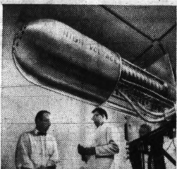
Neutrons generated by this eerie machine help Shell scientists identify metal impurities that sometimes turn up in crude petroleum.
