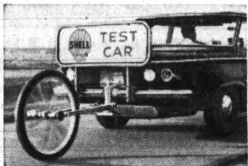
The "fifth wheel." Shell test drivers add a fifth wheel to their cars for precise distance measurement, during mileage tests. It helps them record performance to a decimal point.
