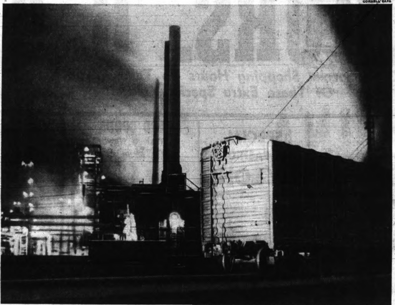
This is where Platformate is made. The "platforming" reactors are primed with a carload of platinum catalyst. During the re-charging process, a tent is erected at the reactor to protect the catalyst from wind and rain. At half-a-million dollars a carload, it is precious stuff.
