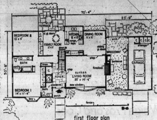
FIRST FLOOR PLAN — There is 1,364 sq. ft. of living comfort on this first floor, including im-
