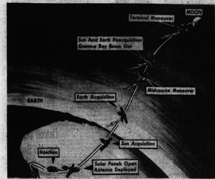
DESTINATION: MOON — Sketch shows the planned 60-hour flight of the Ranger 4 spacecraft to the moon today. Injection is the point at which Ranger goes into a course toward the moon after separating from its Atlas-Agena rocket. At points indicated as earth and sun acquisition and reacquisition Ranger's attitude control system is "locked" onto the earth or sun. The midcourse maneuver is designed to adjust flight to a collision course to the moon.
