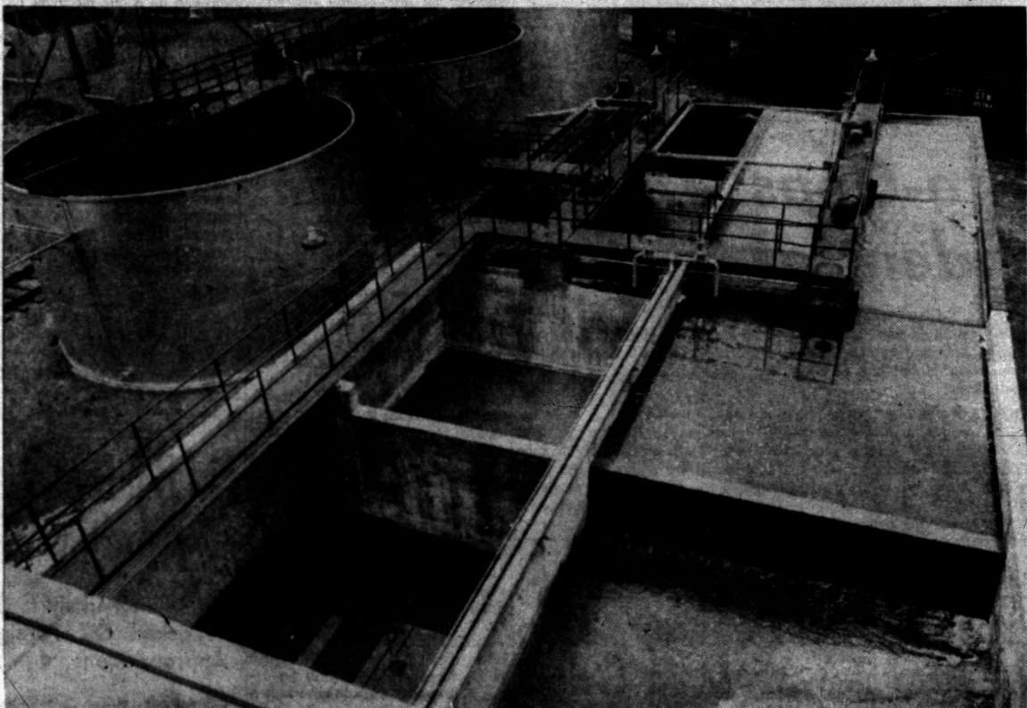
CYANIDE REACTOR —This cyanide reactor is an important segment of the new, giant waste treatment plant at Pontiac Motor Division where 1500 gallons of noxious wastes can be treated each minute. Through an oxidizing process this reactor breaks
