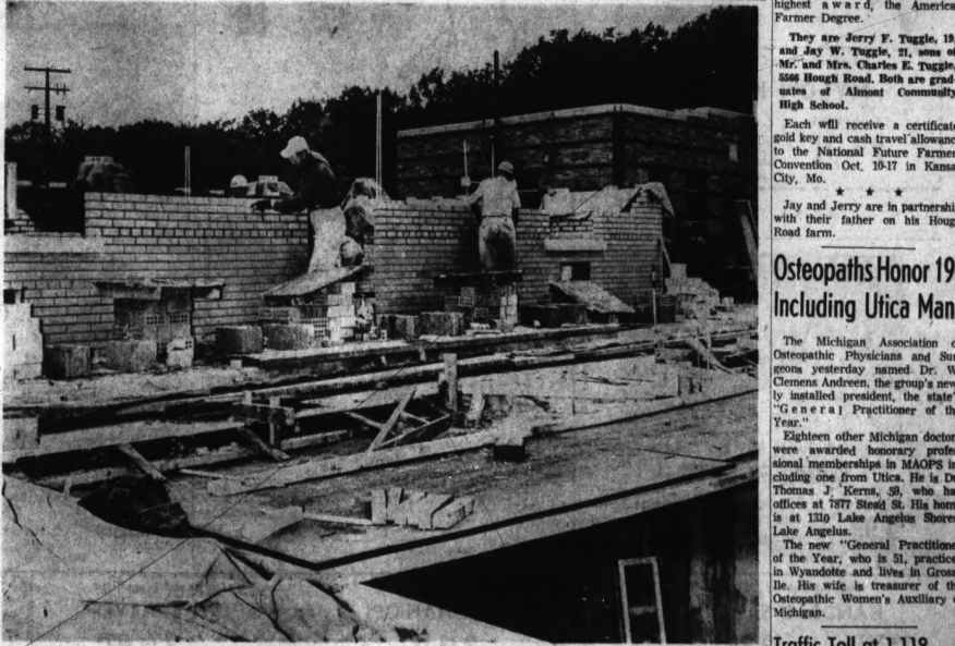
RIGHT ON SCHEDULE — Rochester's project of expanding its sewage treatment plant to double its capacity is nearing the halfway mark toward completion due the middle of March. Workers are pictured here laying the brick for the walls of the blowers building which is one of the main phases of the $425,000 expansion program. The present plant is in the background. When finished, it is expected the facility at the east end of Third Street will serve village needs for the next 30 years. The O. W. Burke Co., Detroit, is general contractor.
