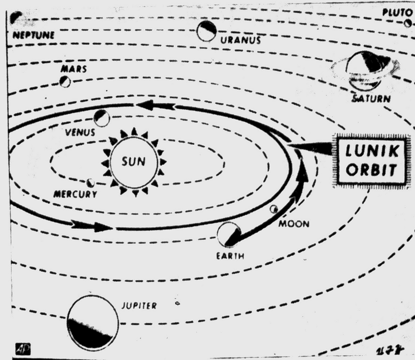
HOW "LUNIK" WOULD ORBIT THE SUN — Arrows and solid line mark how the Russian rocket may orbit the sun like earth and other planets. First arrow along rocket's projected orbital path shows its approximate location now.
