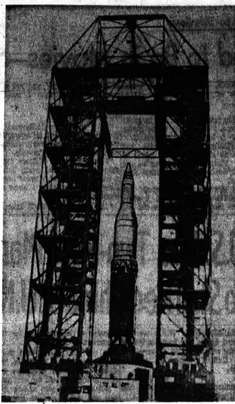
ASSEMBLED SATURN —This three-stage Saturn stands on its launching pad at Cape Canaveral, Fla., where it will be tested on a short flight later this year. The huge vehicle is expected to launch tons of instruments to the moon and Mars by 1965. Pictures were permitted Thursday for the first time.
