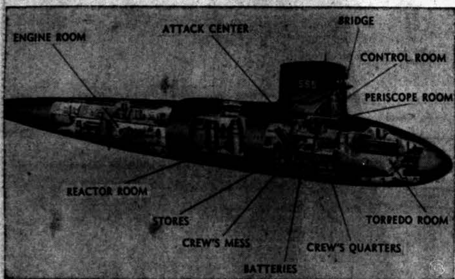
CUTAWAY OF SKIPJACK — Cutaway drawing shows the Skipjack, the Navy's newest nuclear submarine which was launched at Groton, Conn.
