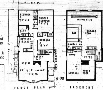
FLOOR PLANS—Architect has packed plenty of living features into the small dimension of this three-bedroom house, including center hall usually seen in larger homes; note excellent division of space in the basement.
