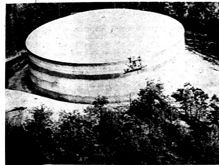
Six-million-gallon ground storage reservoir is an important part of new water system.
