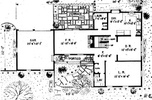
H-87 FIRST FLOOR PLAN
