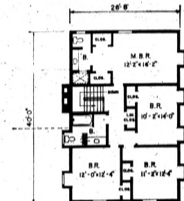
H-87 SECOND FLOOR PLAN
