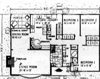
FLOOR PLAN: You can't help but enjoy easy living with a floor plan of this kind, which separates the living and bedroom quarters and permits access to any room without crossing others.
