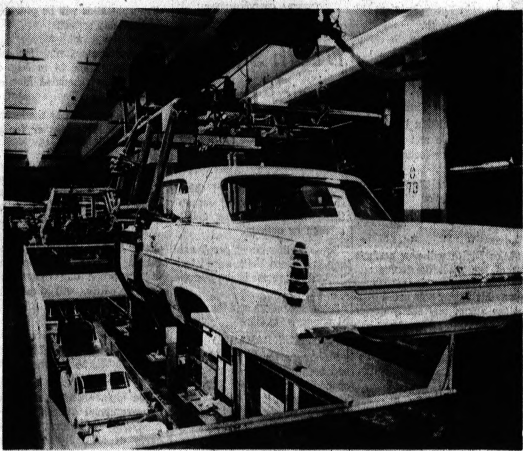
HISTORIC DROP — This two-door Catalina hardtop body being lowered into position at Pontiac Motor Division's final assembly plant was a milestone. It represents the 2,768 car to be assembled yesterday, the highest single-day production total in the division's history. The previous high for one day was 2,638 cars on Oct. 26, 1954. Since the 1963 models were introduced last fall, more than 50,000 have been assembled each month.
