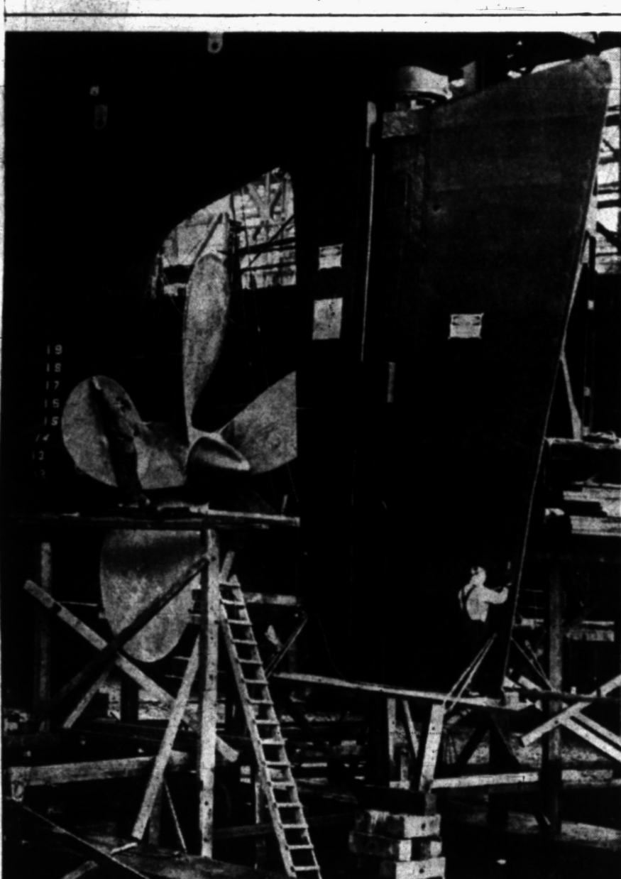
HUGE SCREW—Workmen are shown putting finishing touches on the huge 70,000-pound screw which will drive the recently launched "World Glory," the world's largest tanker. The screw, which will propel the ship at a 20-knot clip, measures 22 1/2 feet in diameter. Built by the Bethlehem Steel Co., the ship will join the Niarchos cargo fleet in April.
