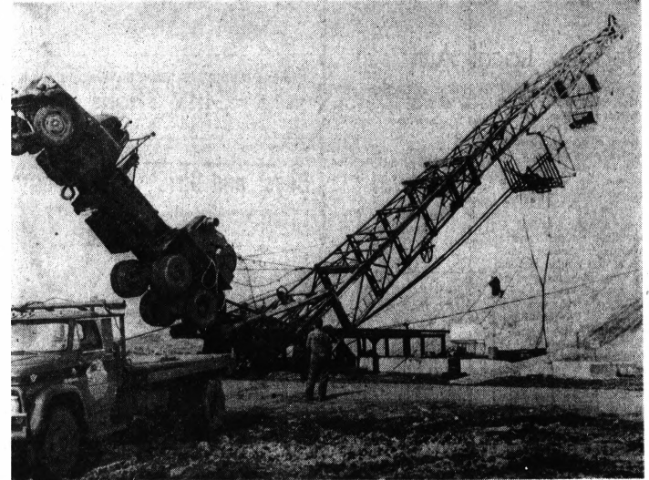
LACK OF SUPPORT — Rear support legs gave out on this oil well tower resulting in this freak accident in Rangely, Colo. A worker on the tower, David Holloway, was not injured when the tower collapsed. Holloway rode the tower down when he was unable to free his safety harness. A 70,000-pound rig was hoisted into the air by the tower.
