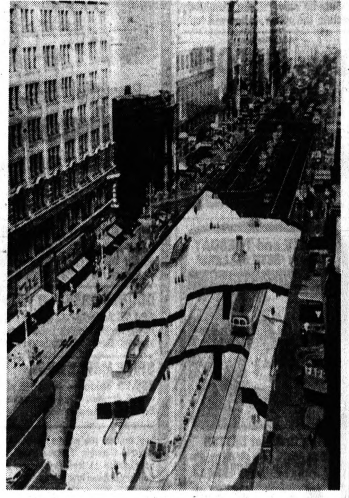
RAIL PLAN —This cutaway sketch in photo of San Francisco's Market Street illustrates proposed modern rail rapid transit system. In the subway plan, high-speed trains will use the lower level. Center level will be used during initial years by streetcars. Upper level will be a pedestrian mezzanine.
