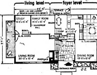
FLOOR PLANS — Expansion portion of this home could be finished by a handy man, adding 517 square feet of living area to home. Foyer and living room levels (ground cover area) contain 1,210 square feet and bedroom level 665 square feet. Basement and garage levels are not shown.
