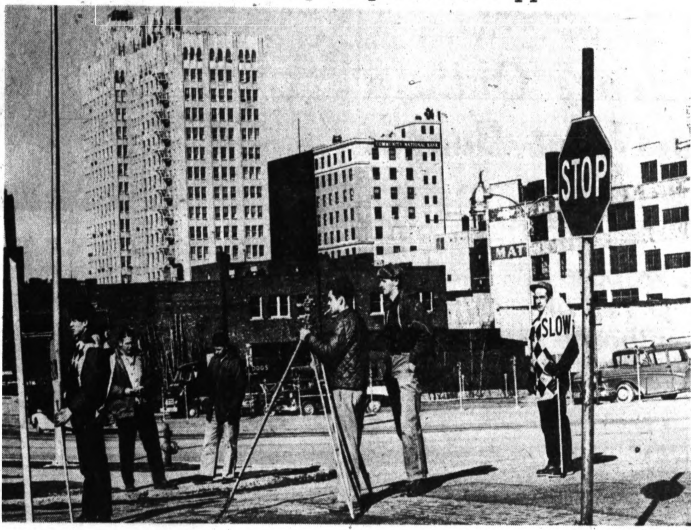
SURVEY LOOP ROUTE — At the corner of East Pike Street in the Civic Center area, a survey team of the State Highway Department plots the future alignment of the downtown loop highway. It is expected that state crews will continue the survey
