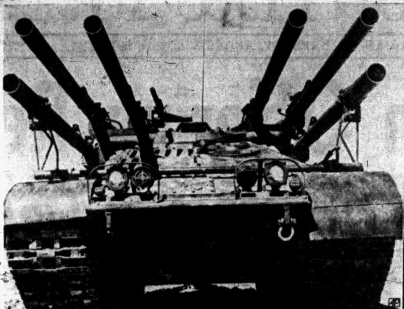
THE THING —The Army and Marine Corps announced August 18 that a $13,000,000 contract has been awarded for this new armored anti-tank vehicle for the Marines. Called Ontos, from the Greek "The Thing," it carries six 106mm recoilless rifles instead of one artillery piece and is lightly armored for speed
